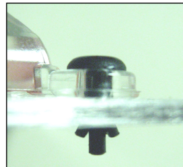
Suggested attachment method with snap rivet through the PCB
